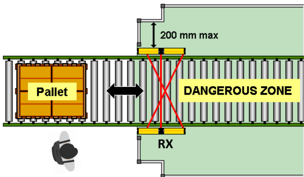
Example of installation with RX right
