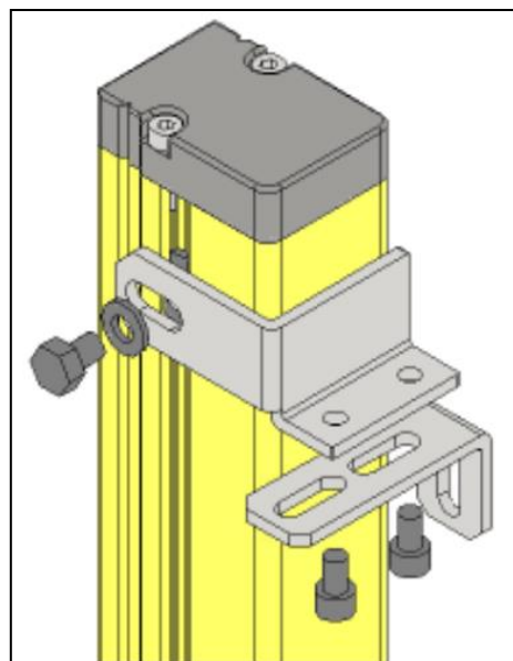
Brackets type STDL mounted
